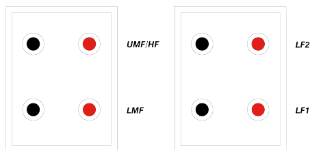
Figure 1: M4 MkII Connector panels, red indicates +ve. The LF panel is nearest the edge of the cabinet.
